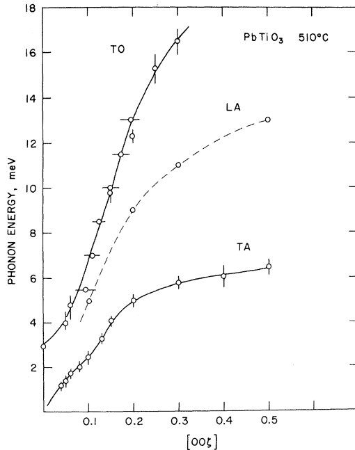
FIG. 1. Three lowest phonon branches in \text{PbTiO}_3 at 510^\circ \text{C} . Vertical error flags indicate constant Q scans. The dip in the acoustic branch is due to the mode coupling as explained in the text.
